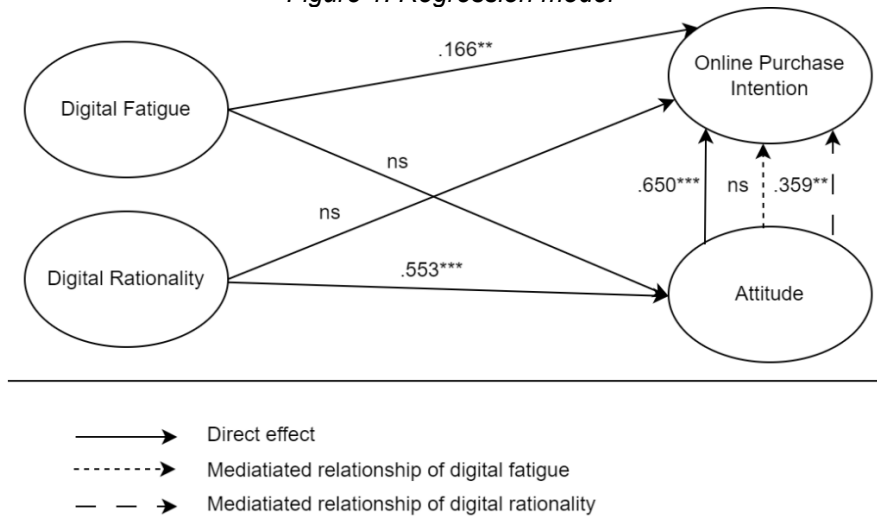
Figure 1: Regression model
